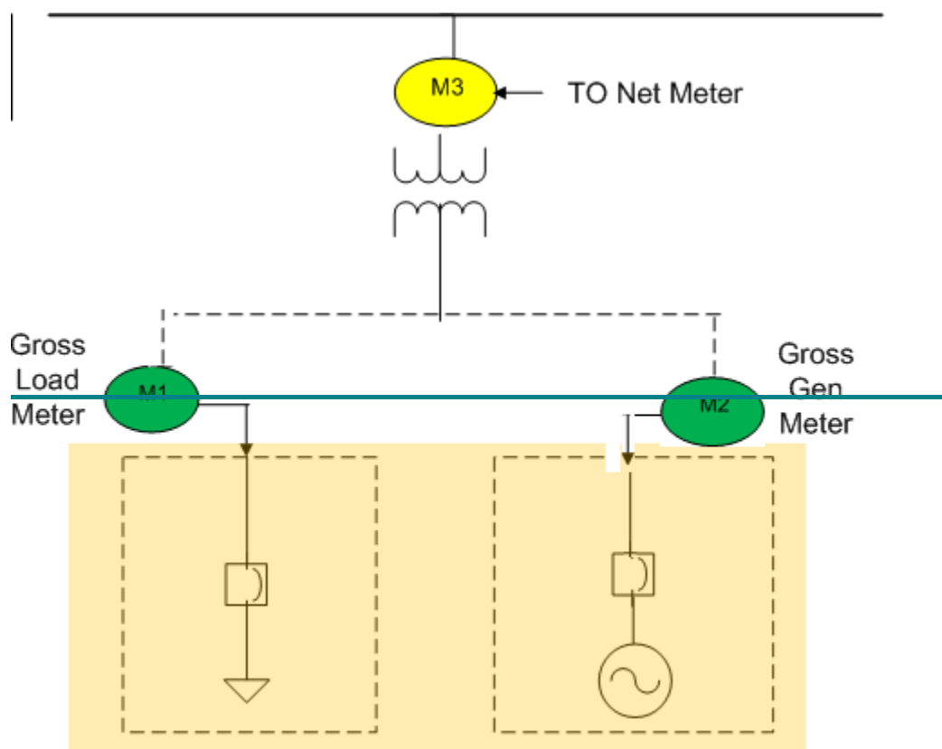
Figure 1: Behind-the-Meter Net Generation Resource Metering Configurations (for illustration purposes only)
